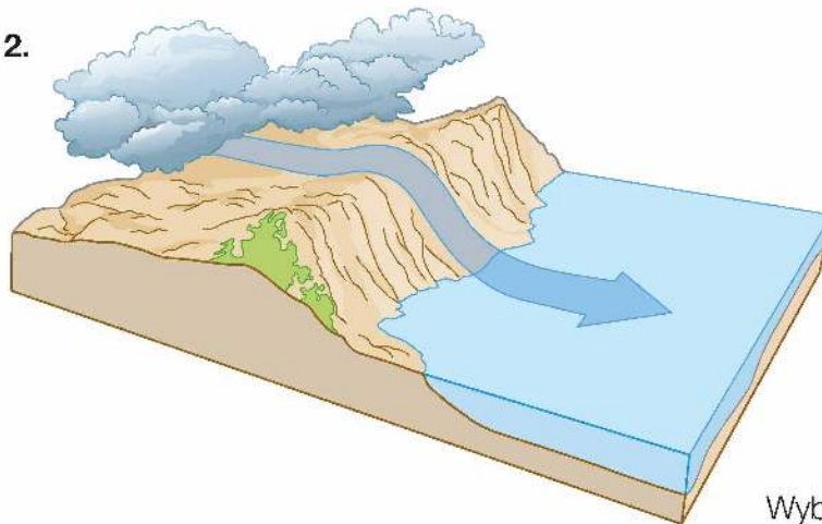
Alpy.
