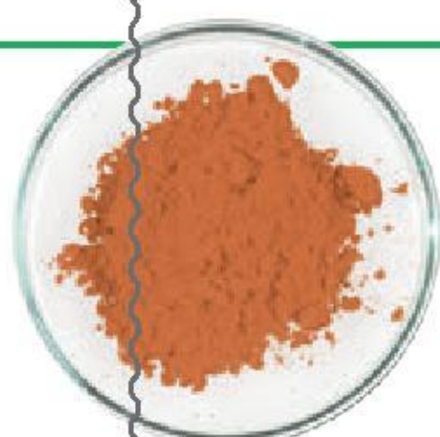
\text{Cu}_2\text{O}
