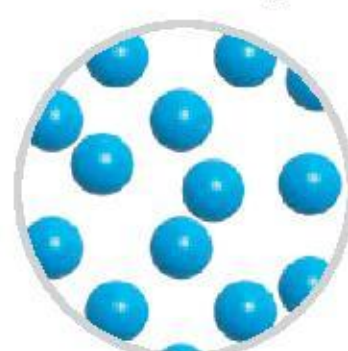
ciecz
