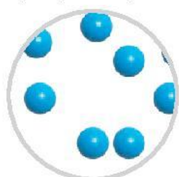
gaz
